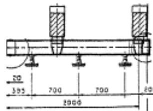
Nozzle Placement
