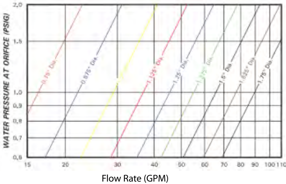
Flow vs pressure Chart
