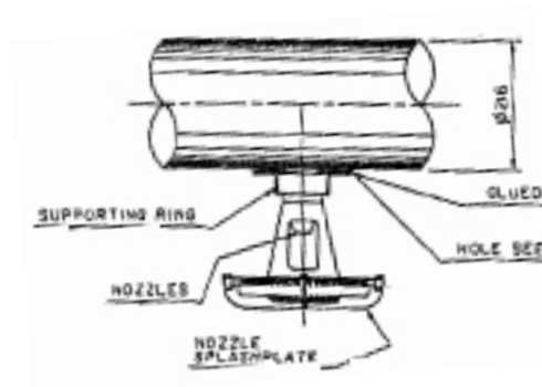
Nozzle Placement
