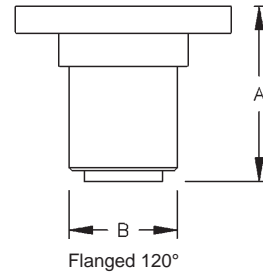
Polypropylene Flange Nozzle
